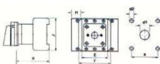
Dimension (Square face switch)
