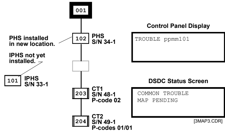
Figure 8-13: Partially restored circuit
